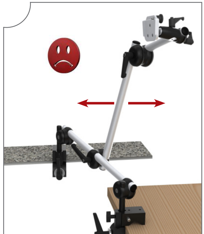
Tightening the lever, prevents the vertical tube from moving side to side.
